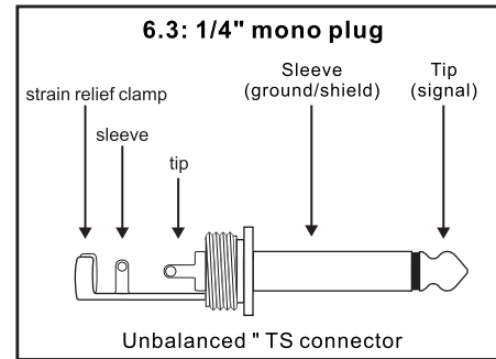
6.3: 1/4" Mono Plug
