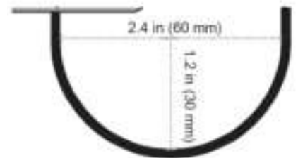
Figure 6. Minimum cable bend radius
