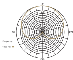
POLAR PATTERN
